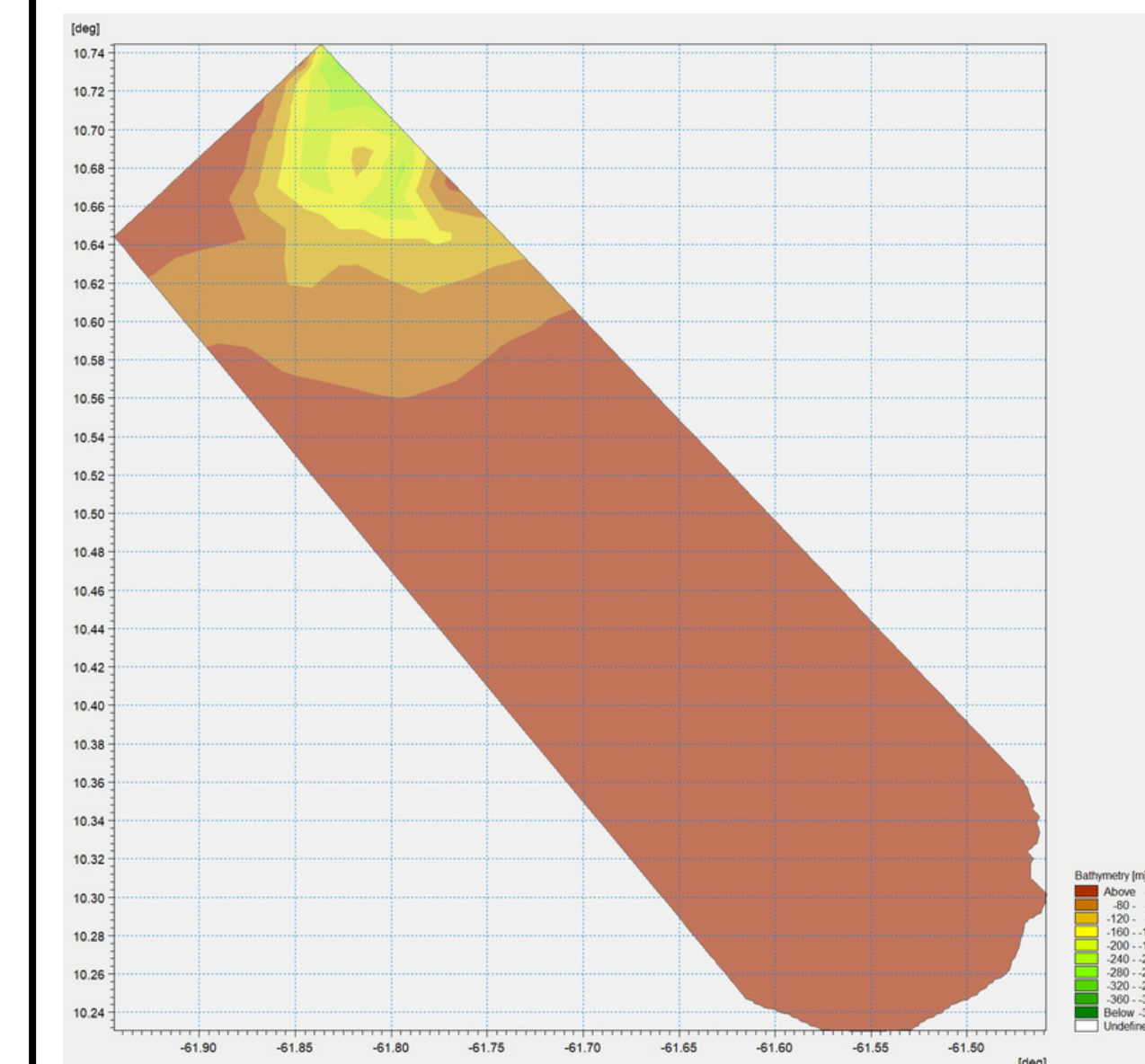
MIKE 21 Domain for Hydrodynamic Modelling
